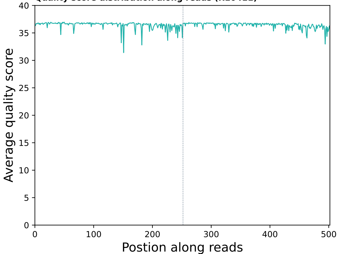
Quality score distribution along reads (R10411)
